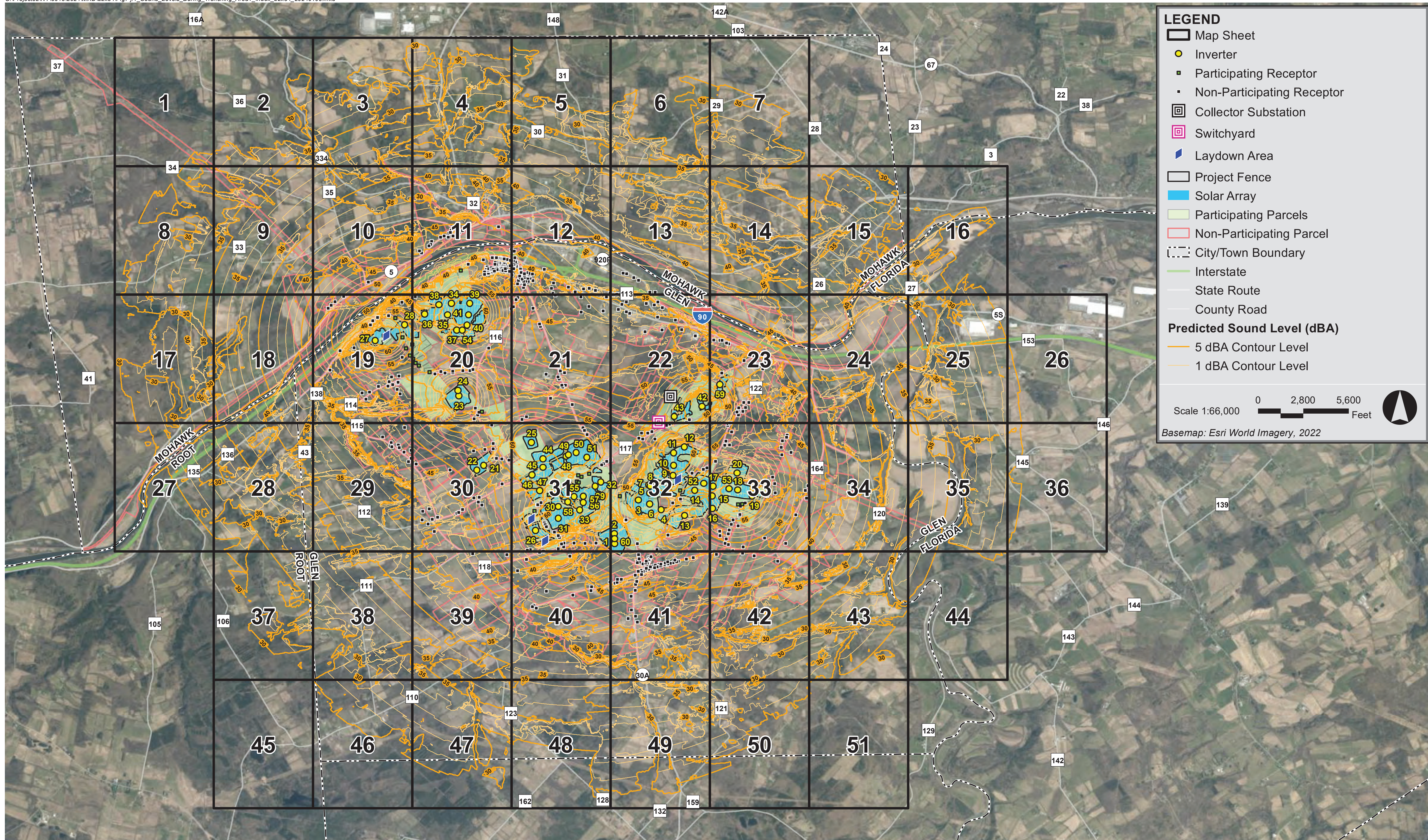
Figure 7-j.1, Index Sound Levels During Simultaneous Trenching & Road Construction – Area 1
